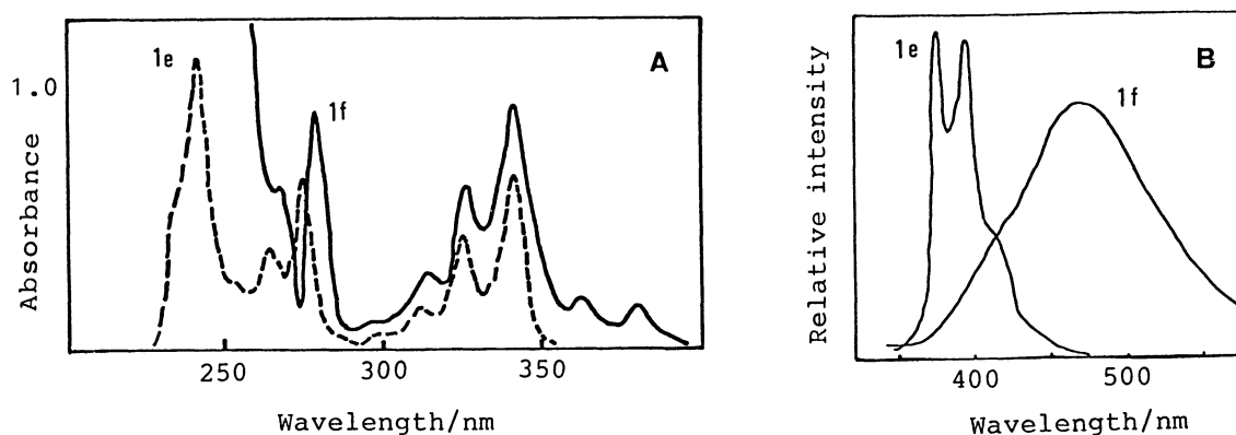
Fig. 2. Absorption (A) and fluorescence (B) spectra of 1e and 1f in methanol.
